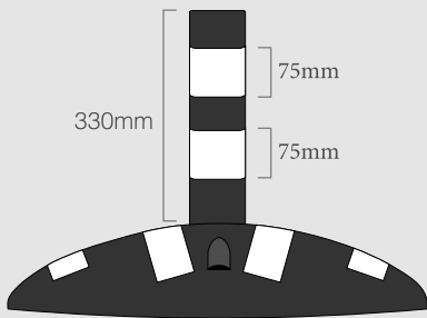
Tiger-Wand 450mm High Product Ref: Low Level - 2 Hoops
